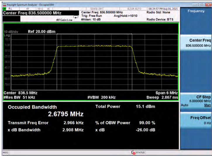
Band5-3MHz-16QAM-20635-15RB#0
