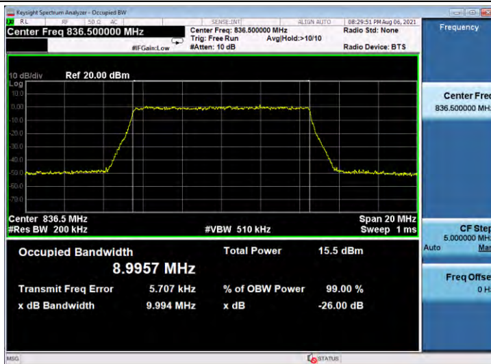
Band5-10MHz-16QAM-20600-50RB#0
