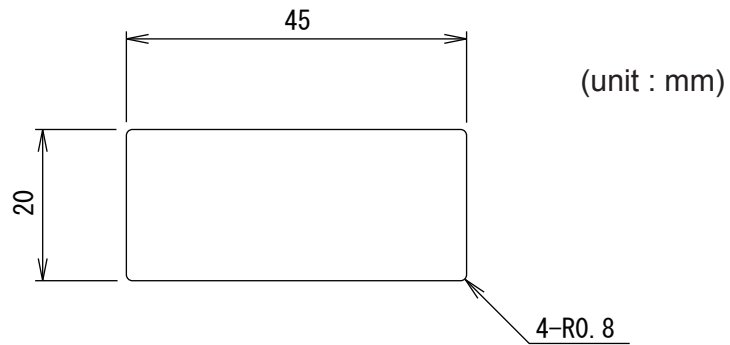
Trimming Die Drawing (S = 1 / 1)
