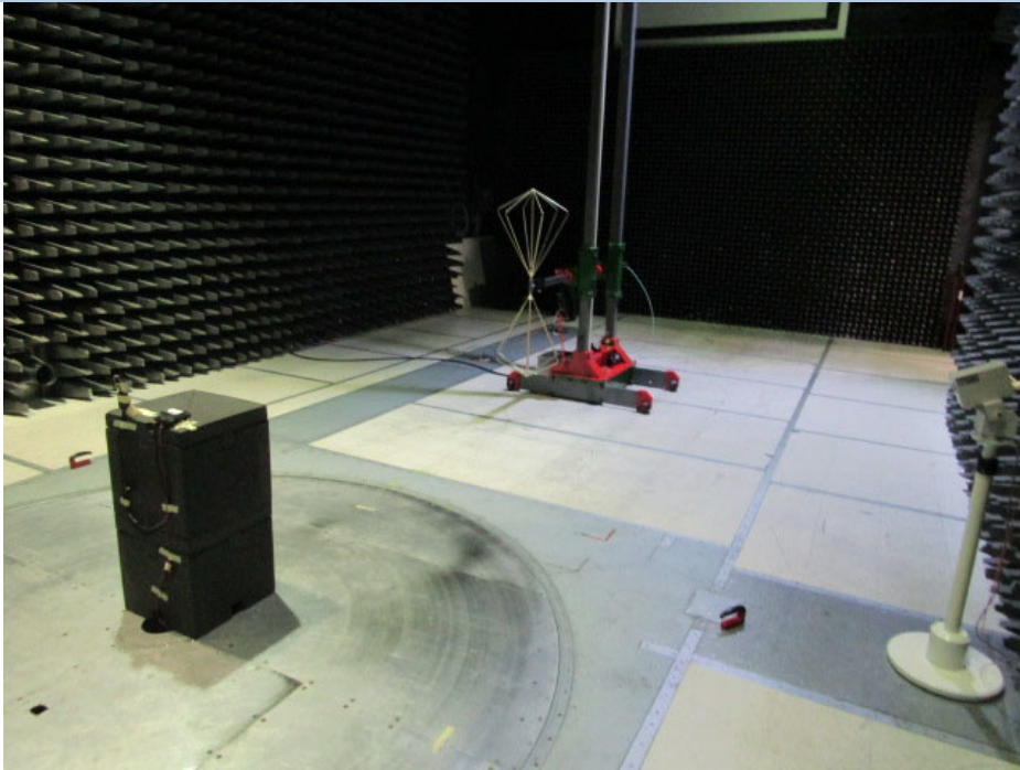
Radiated Emissions
