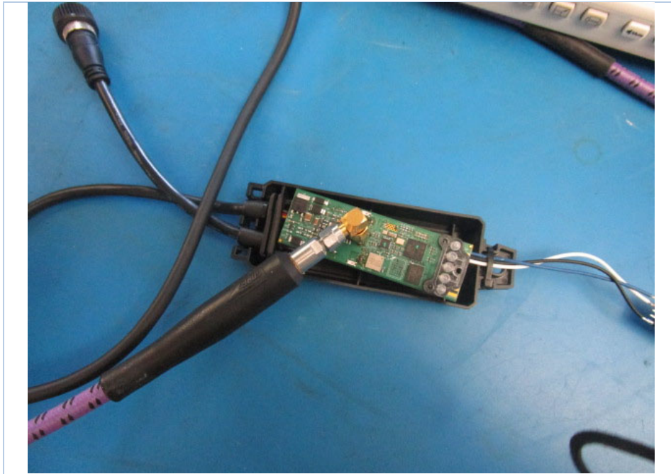
Conducted Setup
