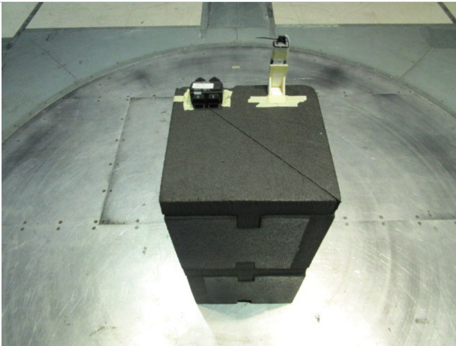
Radiated Emissions
