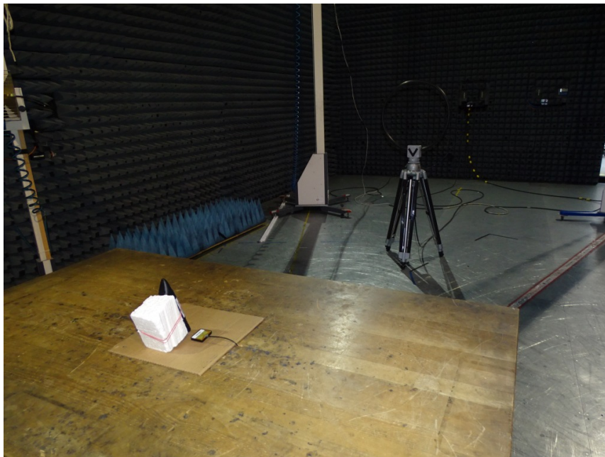
Photo 1 and 2: Test setup for radiated measurements (H-Field, horizontal and vertical)
