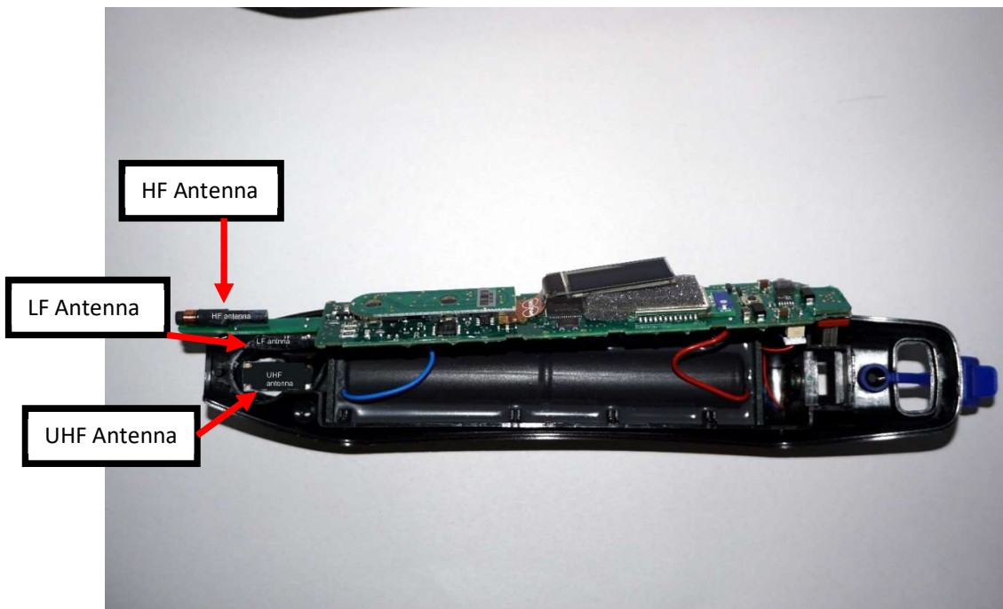
Internal Battery, PCB and antennas
