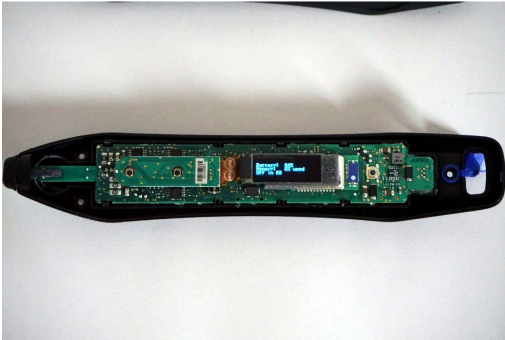
Internal PCB
