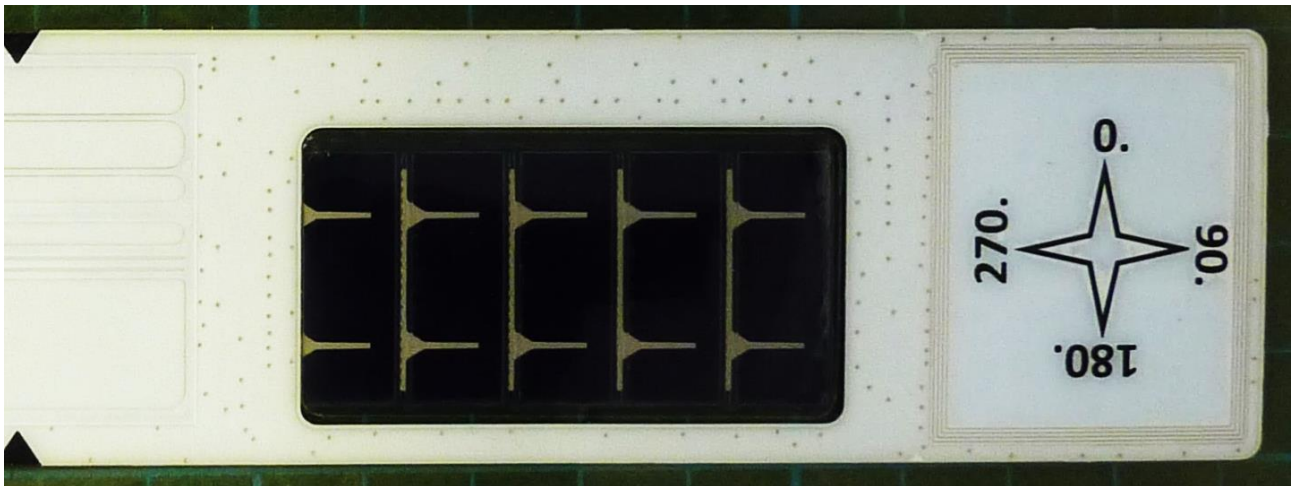
PCB – top view, photovoltaic module
