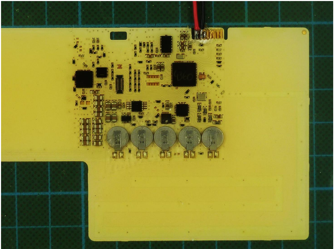
PCB – bottom view, transmitter and integrated antenna
