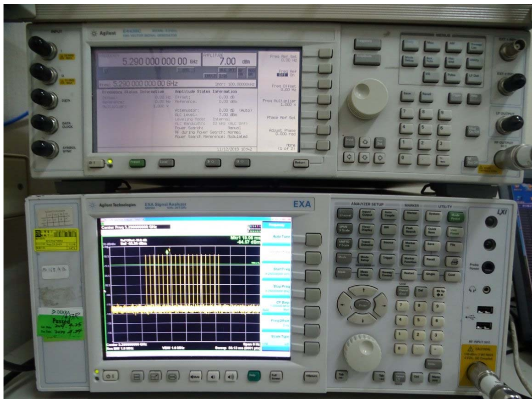
DFS Set-up Photo: Master and Spectrum Analyzer and Radar Generator
