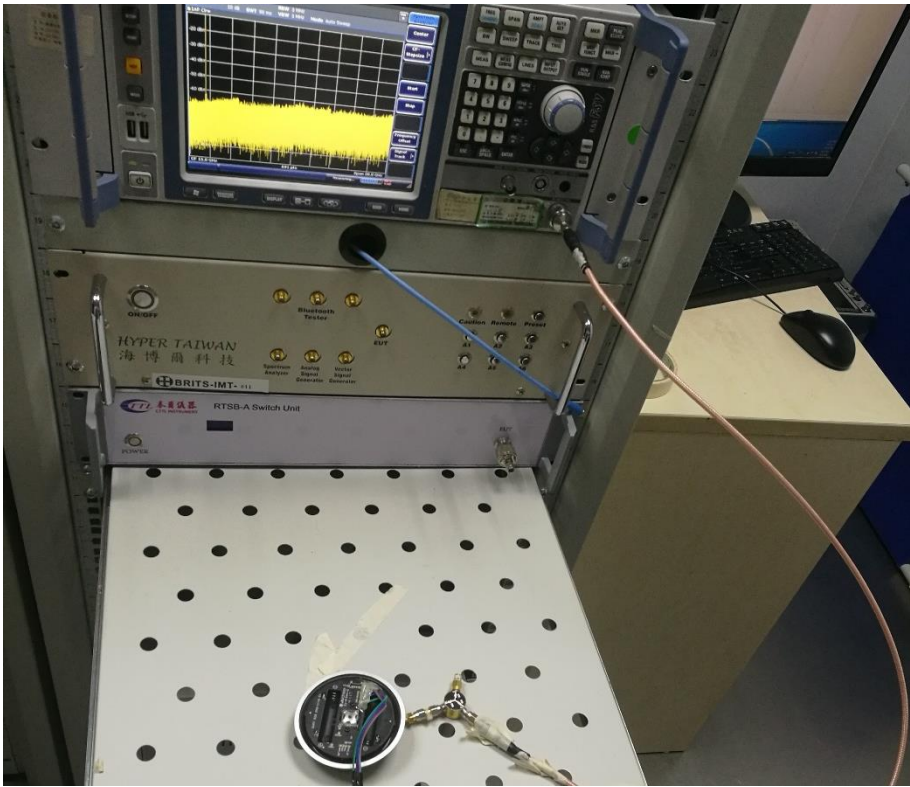
Conducted Test-BLE
