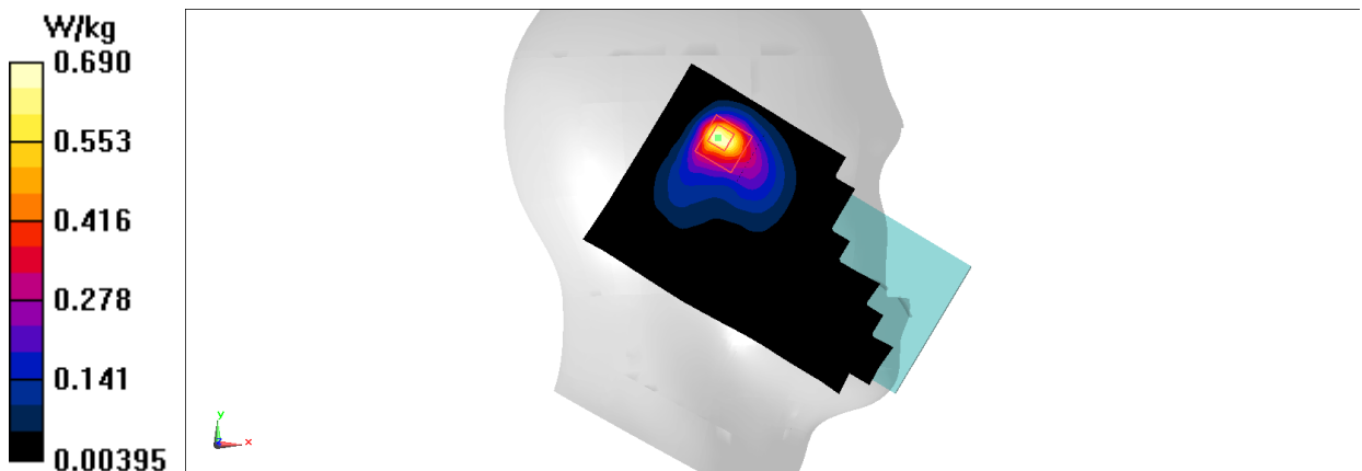
Fig.11 2450 MHz
