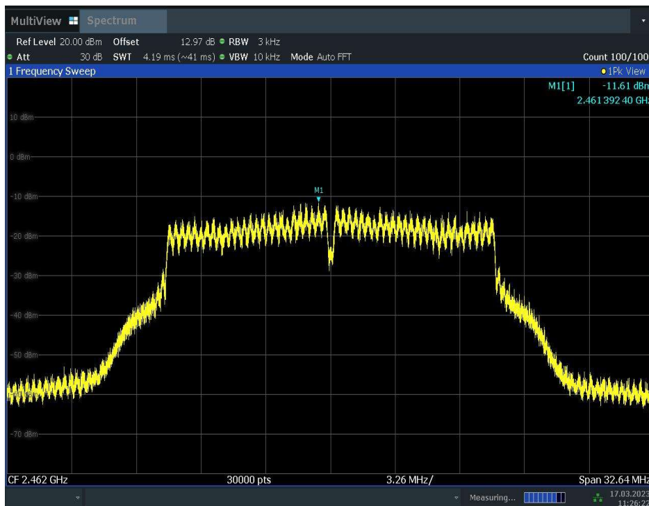
Fig.A.3.12 Power Spectral Density (802.11g, Ch 11)
