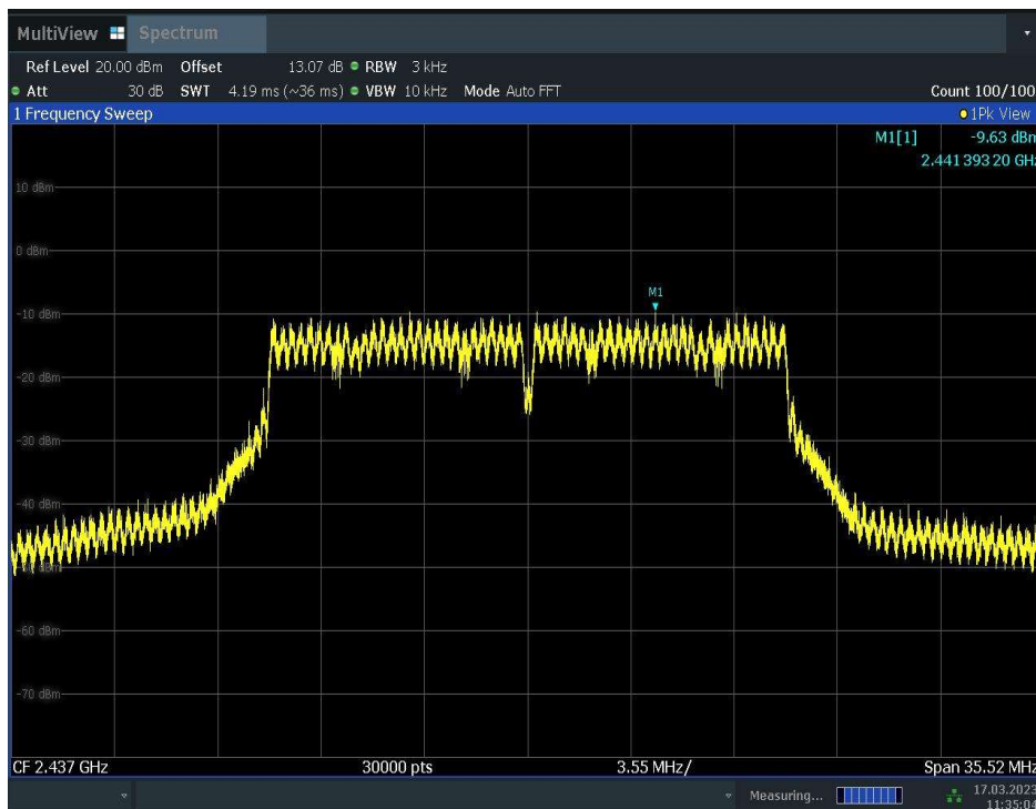
Fig.A.3.14 Power Spectral Density (802.11n-HT20, Ch 6)
