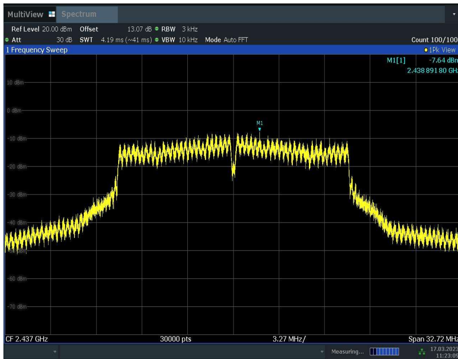
Fig.A.3.11 Power Spectral Density (802.11g, Ch 6)
