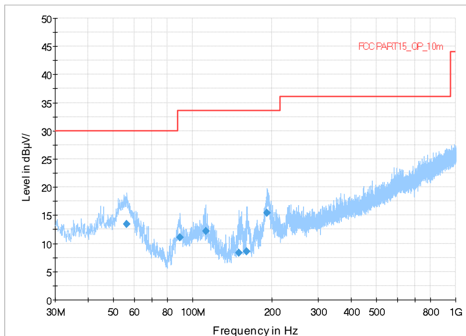
RE FCC_30MHz-1GHz_10m_Direct_testing_FP5b
