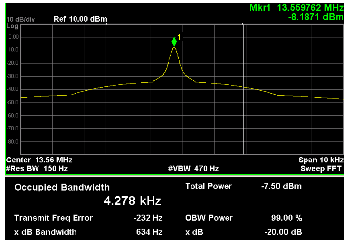
Figure B-10: Measurement results for 20dB Bandwidth
