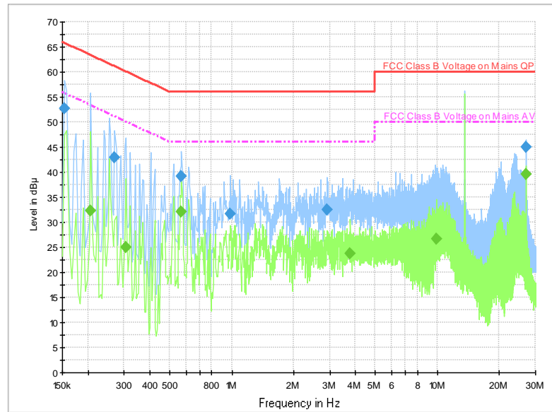
Figure B-12: Measurement results for Conducted Emission
