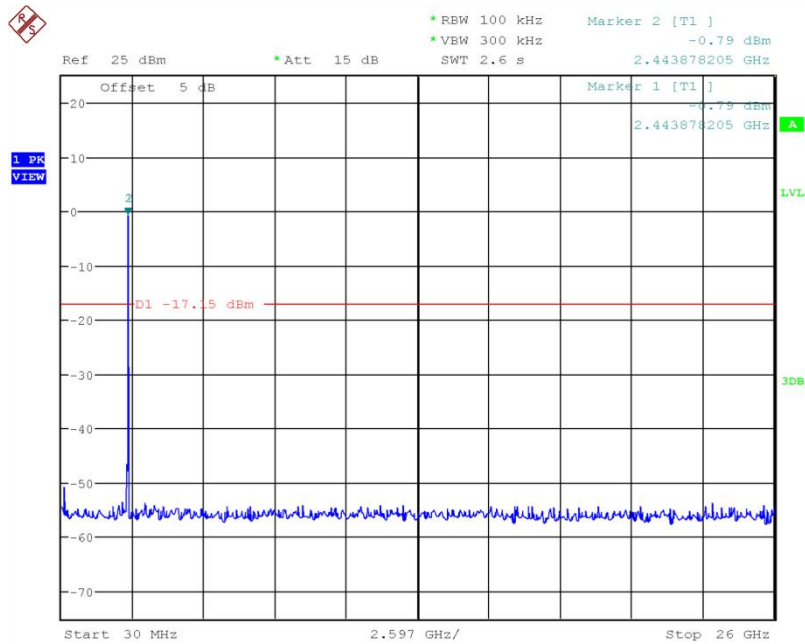
Fig.35 Conducted Spurious Emission (802.11g, Ch11)
