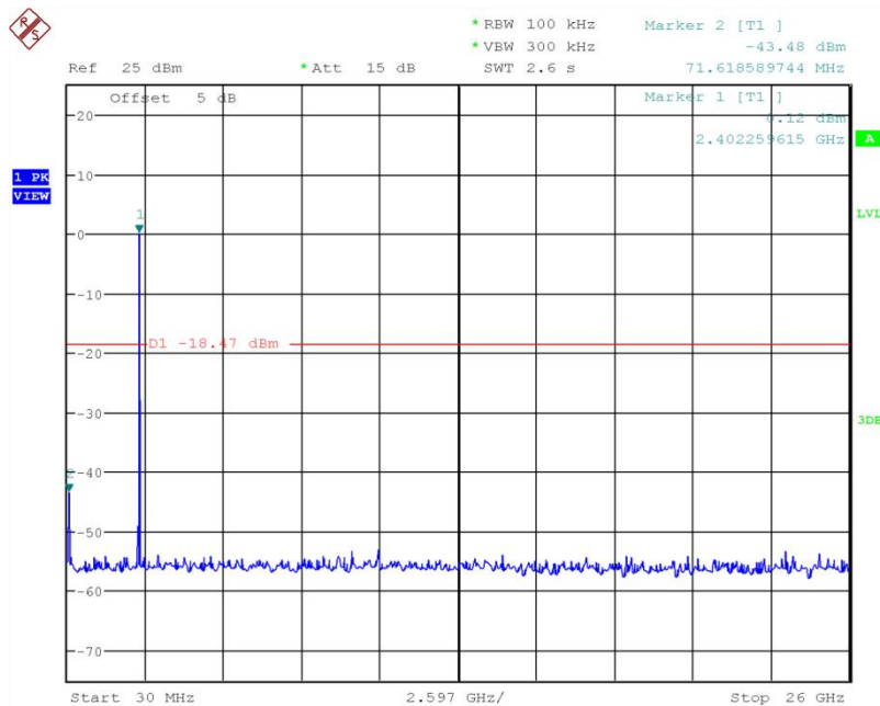
Fig.25 Conducted Spurious Emission (802.11b, Ch1)
