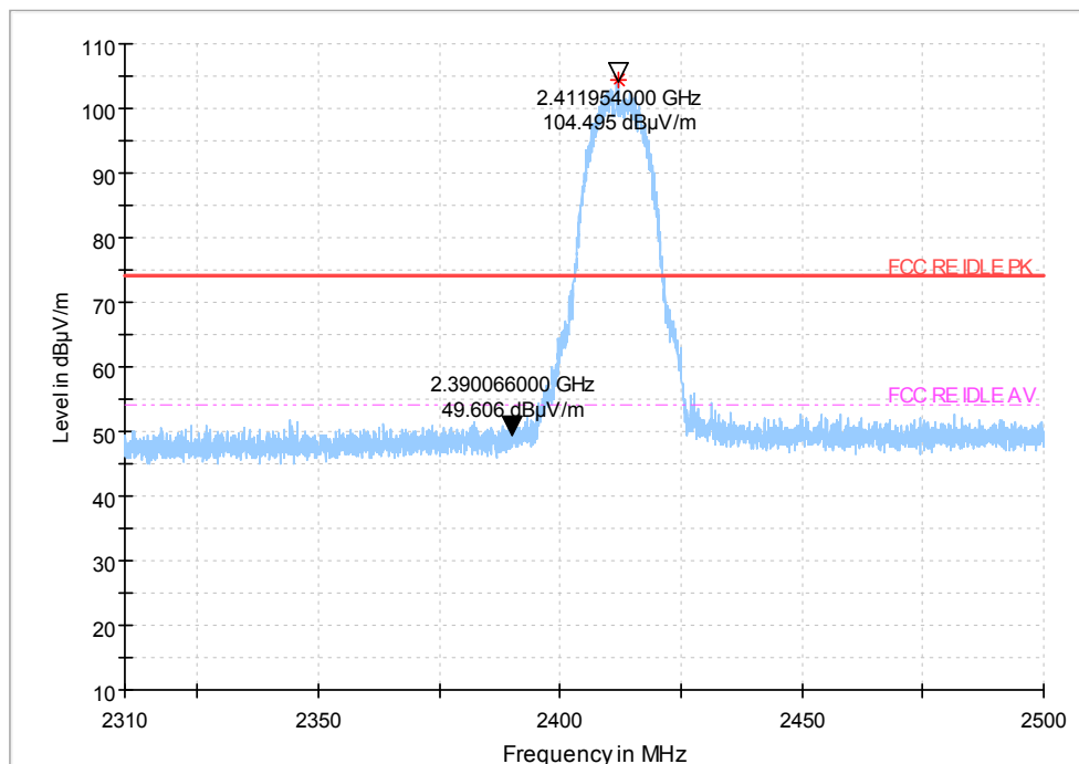
Peak detector
