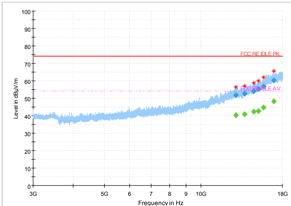
Fig.57 Radiated Spurious Emission (802.11 n-20MHz,Ch11,3GHz~18GHz)
