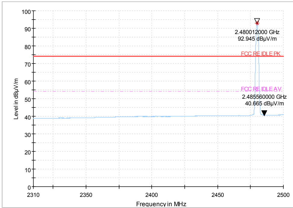
Fig.54 Radiated emission (Power): 8DPSK, high channel
