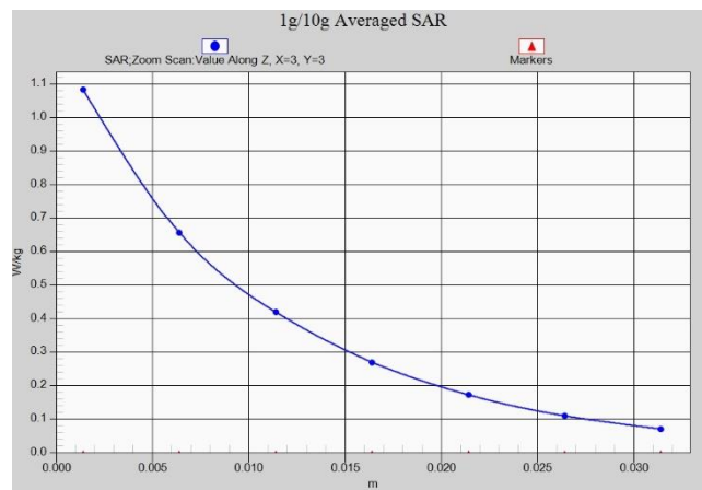
Fig. 1-57 Z-Scan at power reference point (n66)
