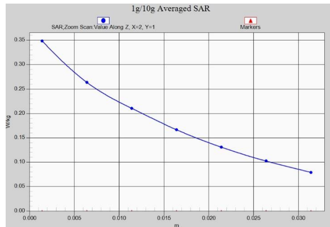
Fig. 1-63 Z-Scan at power reference point (n71)
