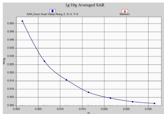
Fig. 1-29 Z-Scan at power reference point (LTE Band38)
