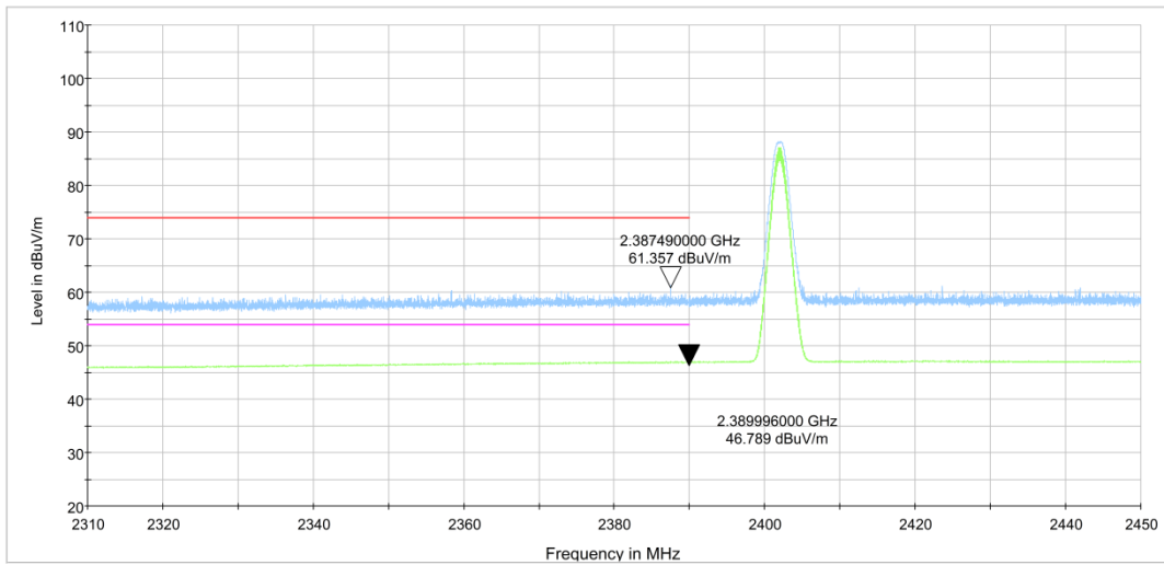
Fig.3. Frequency Band Edges: GFSK, 2402 MHz, Hopping Off, 2.31 GHz – 2.45GHz
