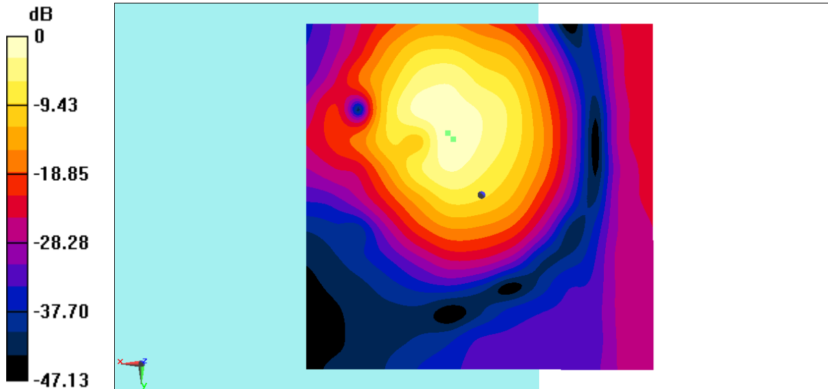
Fig B.4 T-Coil LTEB2
