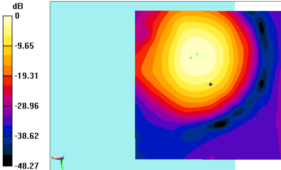
Fig B.2 T-Coil WiFi2.4G
