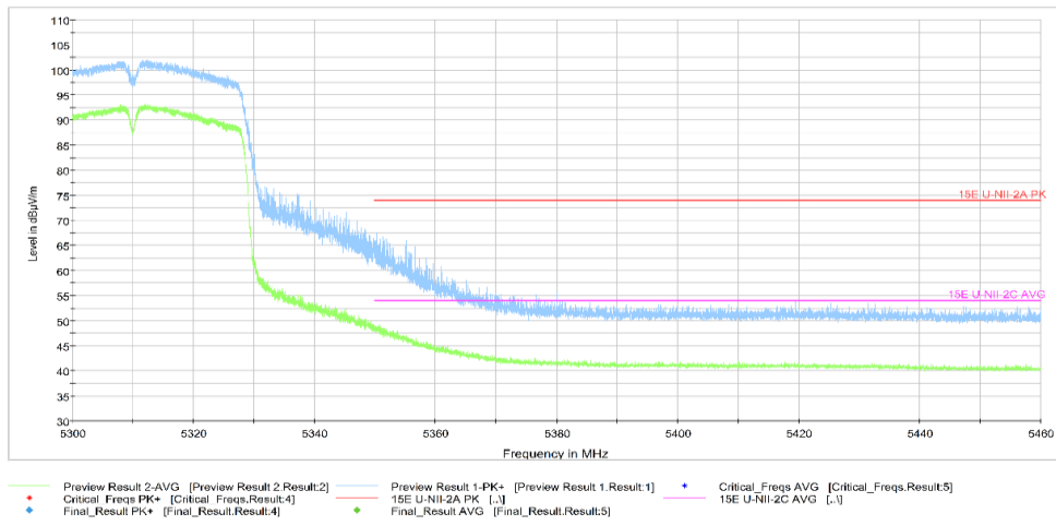
Fig.51 Band Edges (802.11ac-HT40 Ch62, 5310MHz)
