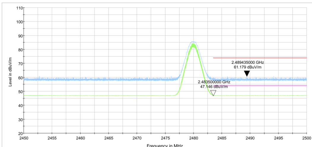
Fig.4. Frequency Band Edges: GFSK, 2480 MHz, Hopping Off, 2.45 GHz - 2.50GHz
