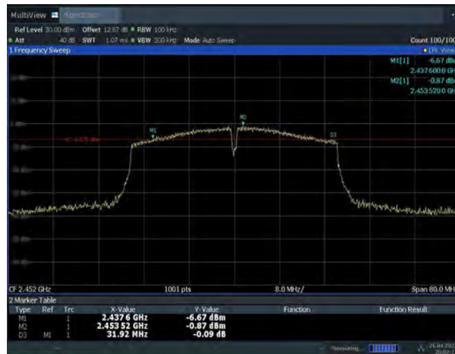
Fig.A.4.12 Occupied 6dB Bandwidth (802.11n-HT40, Ch 9)
