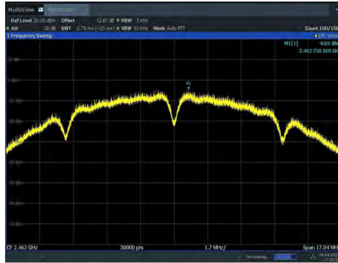
Fig.A.3.3 Power Spectral Density (802.11b, Ch 11)
