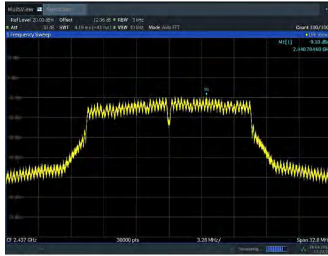
Fig.A.3.5 Power Spectral Density (802.11g, Ch 6)
