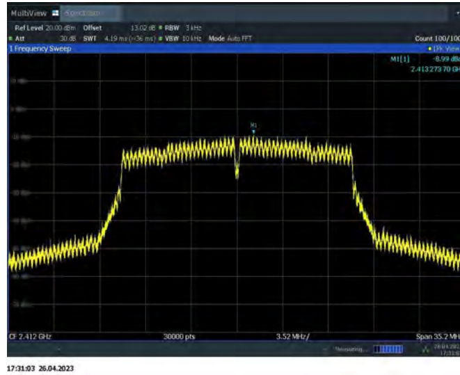
Fig.A.3.7 Power Spectral Density (802.11n-HT20, Ch 1)
