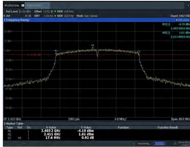
Fig.A.4.7 Occupied 6dB Bandwidth (802.11n-20MHz, Ch 1)
