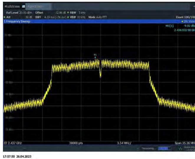
Fig.A.3.8 Power Spectral Density (802.11n-HT20, Ch 6)
