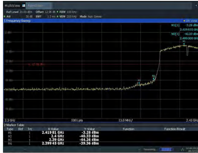
Fig.A.5.7 Band Edges (802.11n-HT40, Ch 3)
