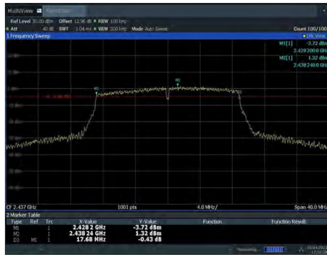
Fig.A.4.8 Occupied 6dB Bandwidth (802.11n-HT20, Ch 6)
