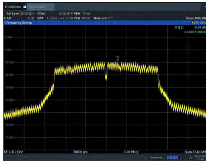
Fig.A.3.4 Power Spectral Density (802.11g, Ch 1)
