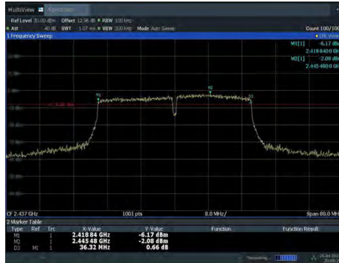
Fig.A.4.11 Occupied 6dB Bandwidth (802.11n-HT40, Ch 6)
