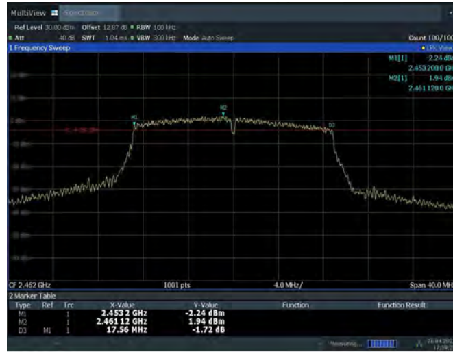
Fig.A.4.9 Occupied 6dB Bandwidth (802.11n-HT20, Ch 11)
