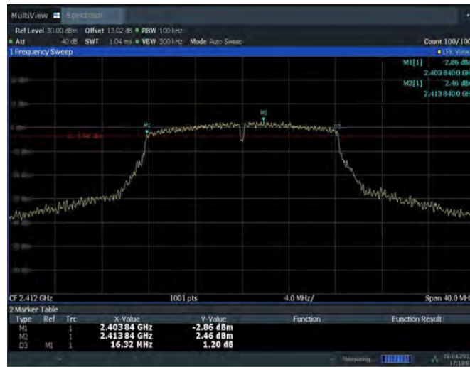
Fig.A.4.4 Occupied 6dB Bandwidth (802.11g, Ch 1)
