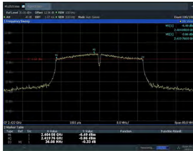
Fig.A.4.10 Occupied 6dB Bandwidth (802.11n-40MHz, Ch 3)
