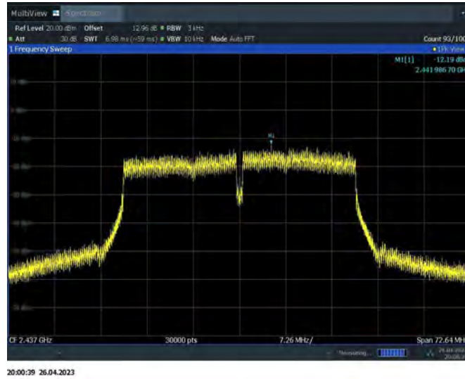
Fig.A.3.11 Power Spectral Density (802.11n-HT40, Ch 6)
