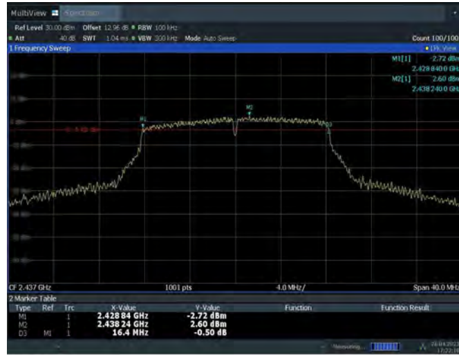
Fig.A.4.5 Occupied 6dB Bandwidth (802.11g, Ch 6)
