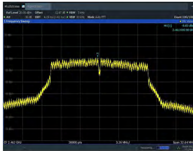
Fig.A.3.6 Power Spectral Density (802.11g, Ch 11)
