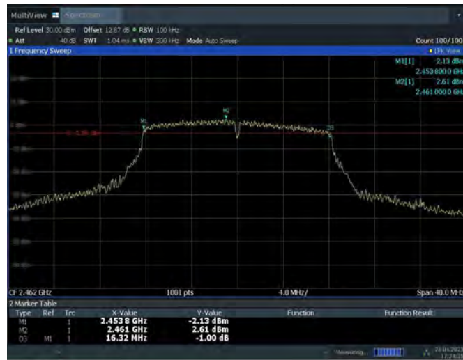
Fig.A.4.6 Occupied 6dB Bandwidth (802.11g, Ch 11)
