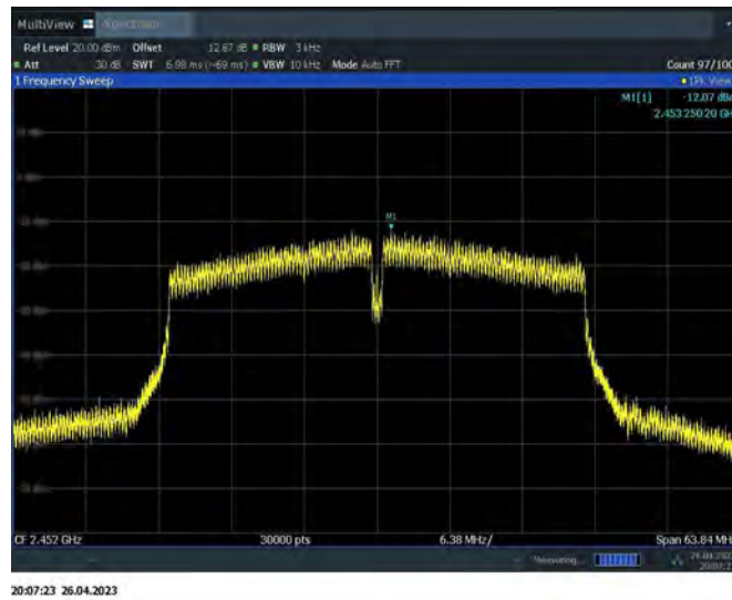
Fig.A.3.12 Power Spectral Density (802.11n-HT40, Ch 9)
