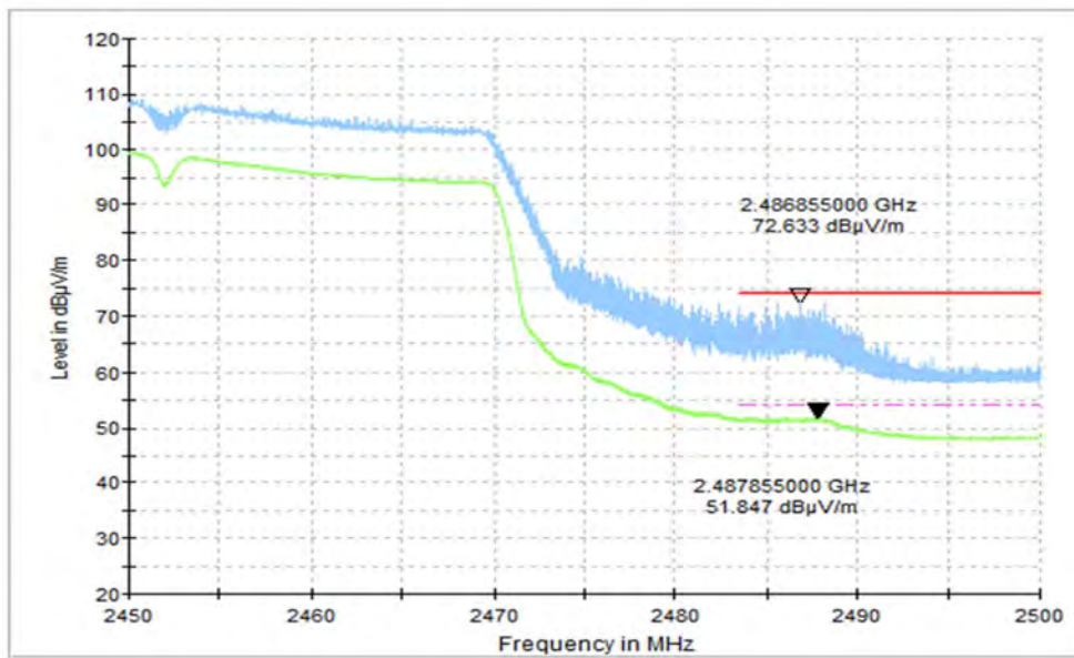
Fig.A.6.2.10 Transmitter Spurious Emission - Radiated (Power): 802.11n-HT40, ch9, 2.45 GHz - 2.50GHz
