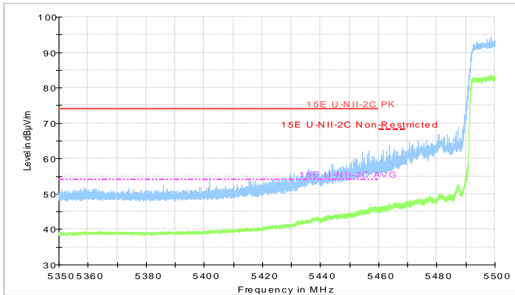
Fig.54 Band Edges (802.11ac-HT80 Ch106, 5530MHz)
