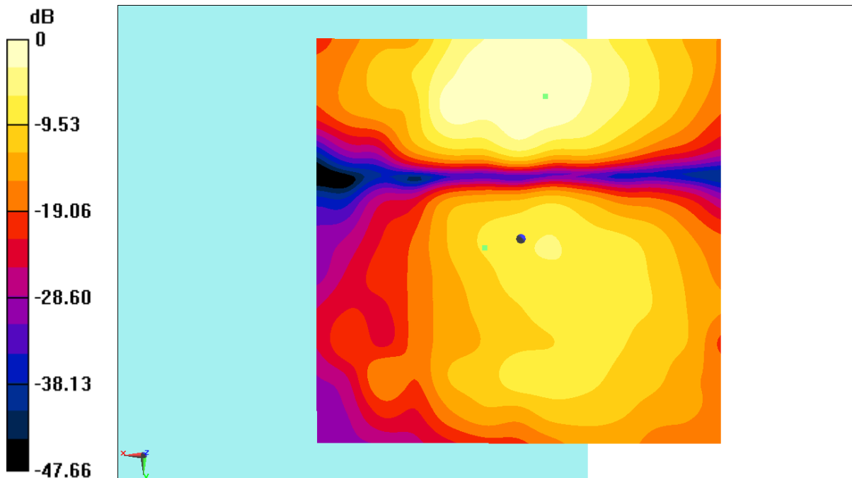
Fig B.1 T-Coil WiFi-5G
