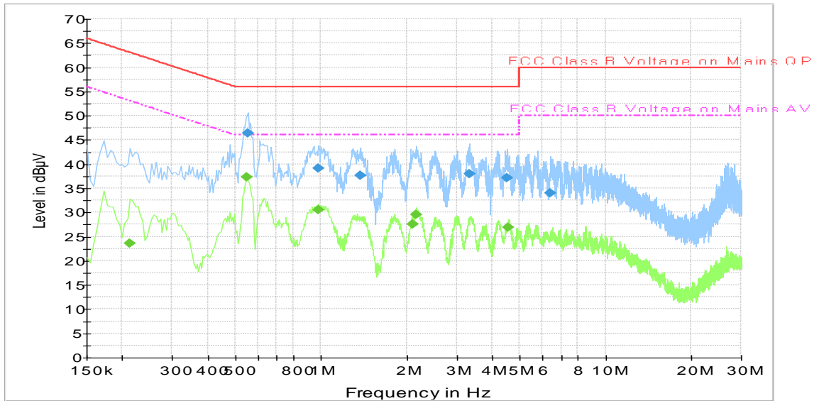
Fig.B.9.1 AC Powerline Conducted Emission- bluetooth
