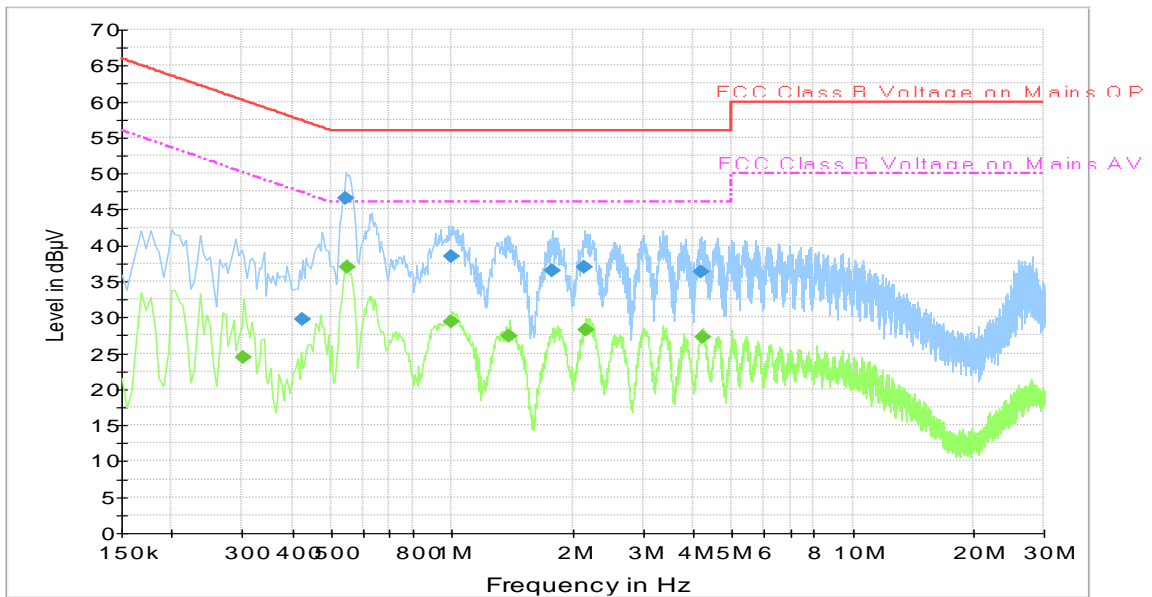
Fig.B.9.2 AC Powerline Conducted Emission-Idle
