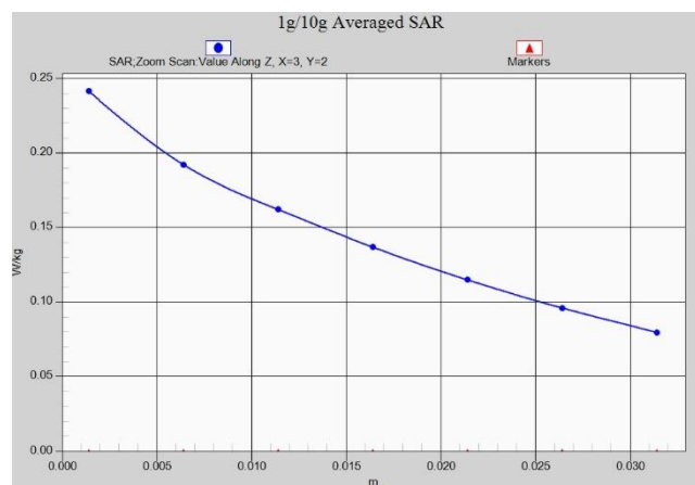
Fig. 1-11 Z-Scan at power reference point (LTE Band12)
