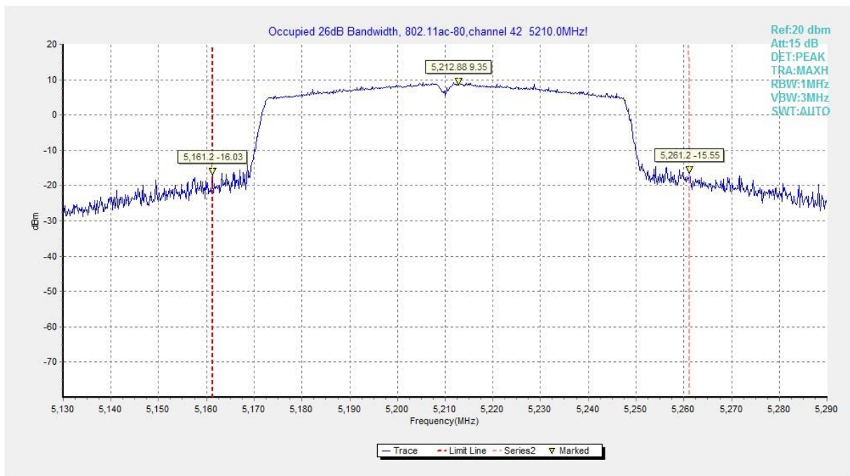
Fig.28 Occupied 26dB Bandwidth (802. 11ac-HT80, 5210MHz)
