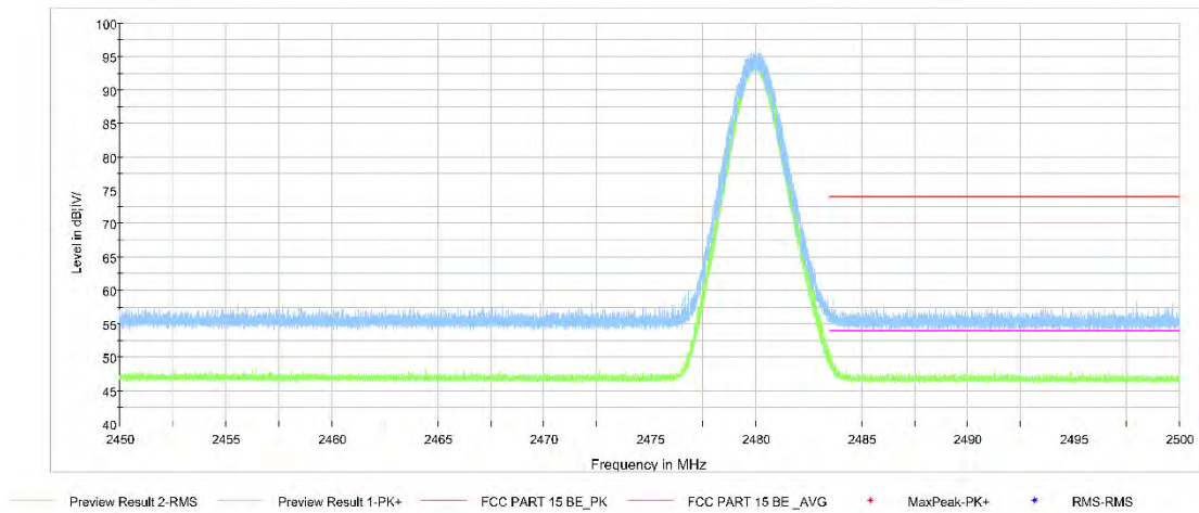
Fig.18. Frequency Band Edges: 8DPSK, Channel 78, 2.45 GHz - 2.50GHz
