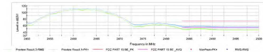
Fig.A.6.2.2 Transmitter Spurious Emission - Radiated (Power): 802.11b, ch11, 2.45 GHz - 2.50GHz
