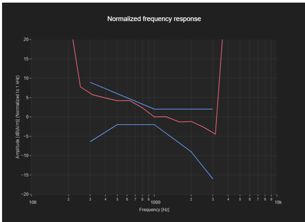
Figure C.2 Frequency Response of VoNR N41
