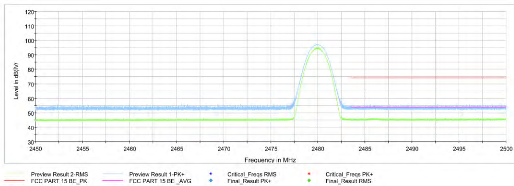
Fig.63. Frequency Band Edges: 8DPSK, Channel 78, 2.45 GHz - 2.50GHz
