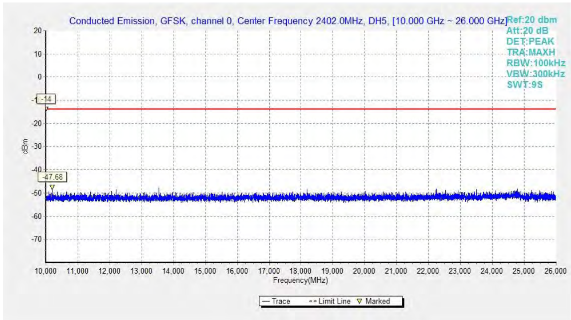
Fig.17. Conducted spurious emission: GFSK, Channel 0, 10GHz - 26GHz
