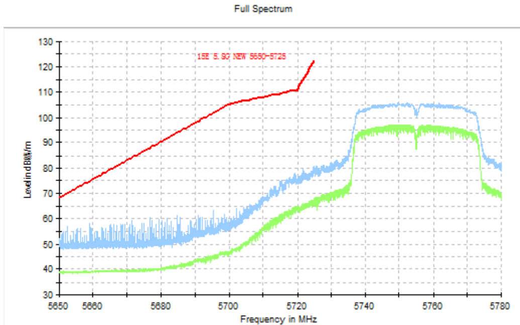
Fig. 19 Band Edges (802.11n-HT40, 5755MHz)
