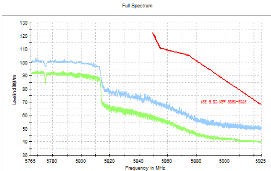
Fig. 26 Band Edges (802.11ac-HT80, 5775MHz)
