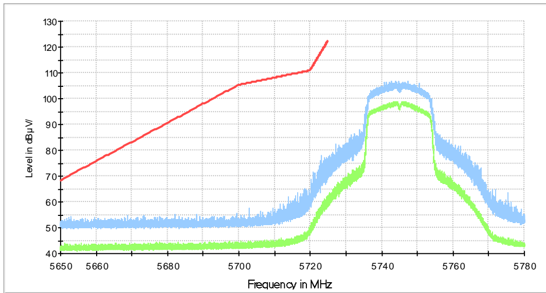
Fig. 14 Band Edges (802.11ac-HT20, 5745MHz)
