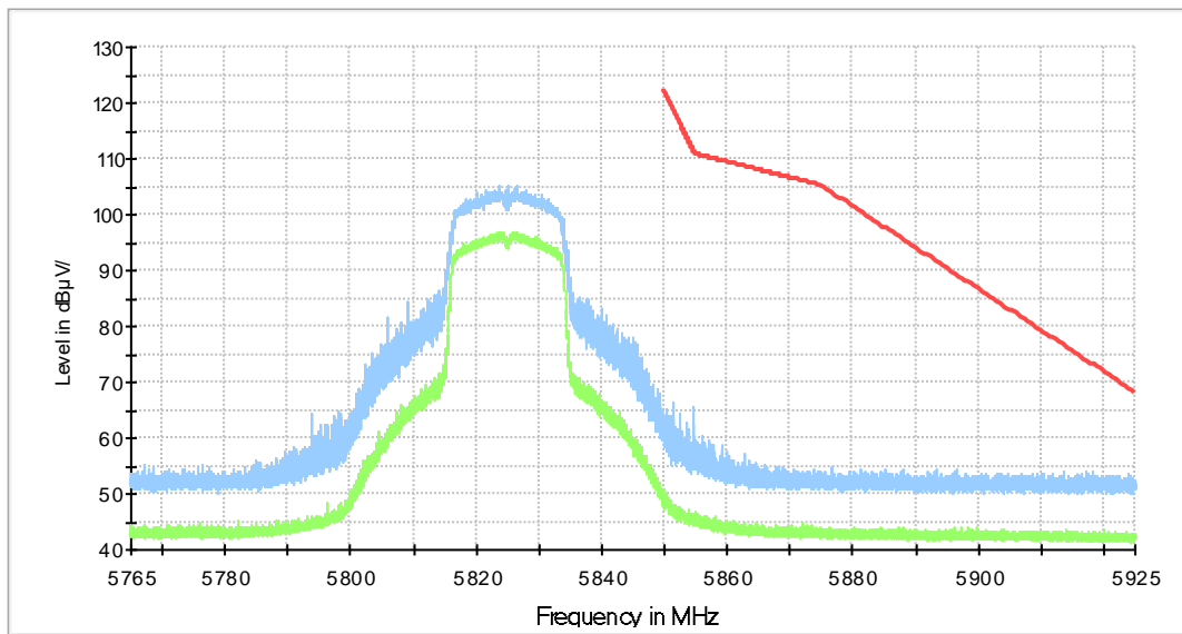
Fig. 15 Band Edges (802.11ac-HT20, 5825MHz)
