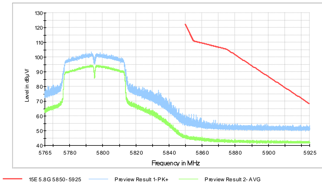
Fig. 17 Band Edges (802.11n-HT40, 5795MHz)
