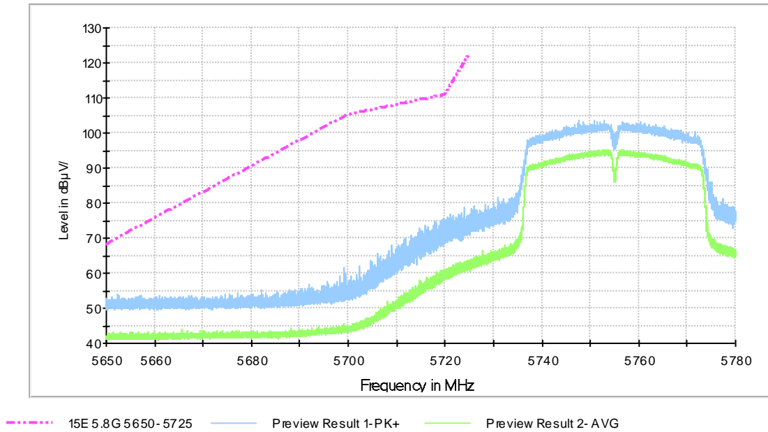
Fig. 16 Band Edges (802.11n-HT40, 5755MHz)
