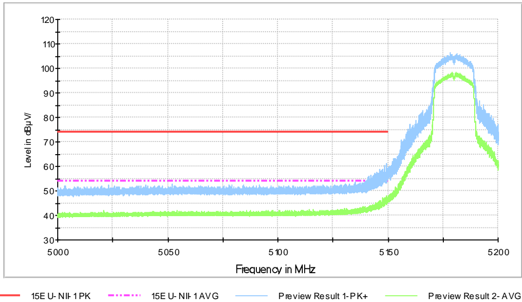
Fig.42 Band Edges (802.11ac-HT20, 5180MHz)
