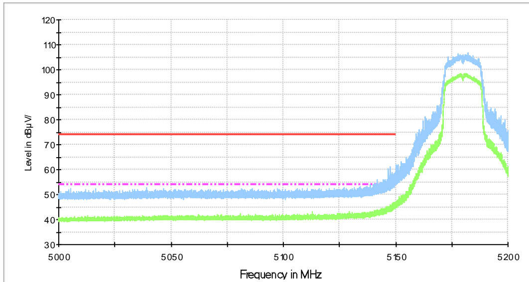
Fig.34 Band Edges (802.11a, 5180MHz)
