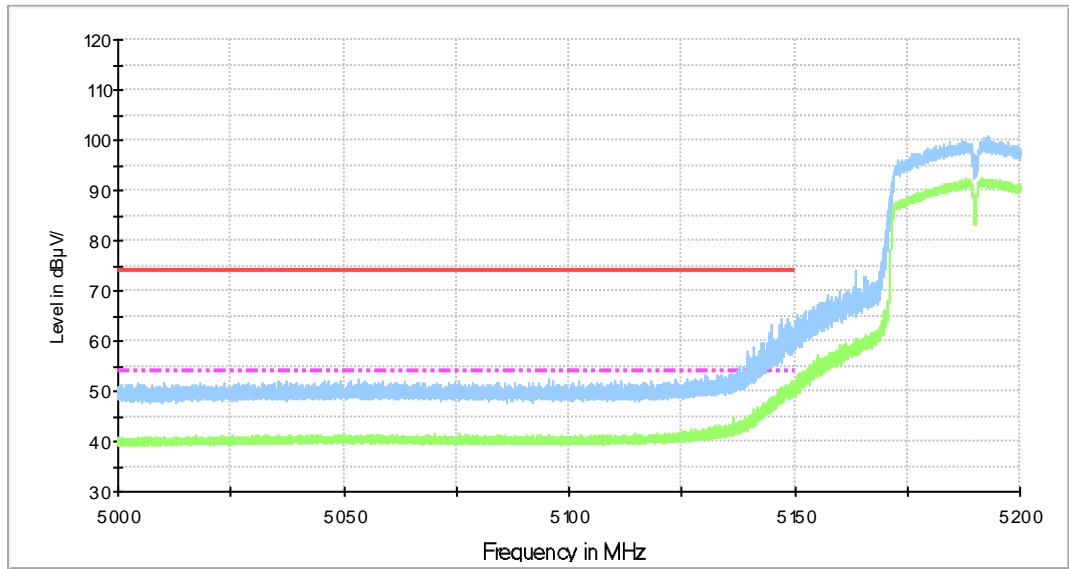
Fig.46 Band Edges (802.11n-HT40, 5190MHz)
