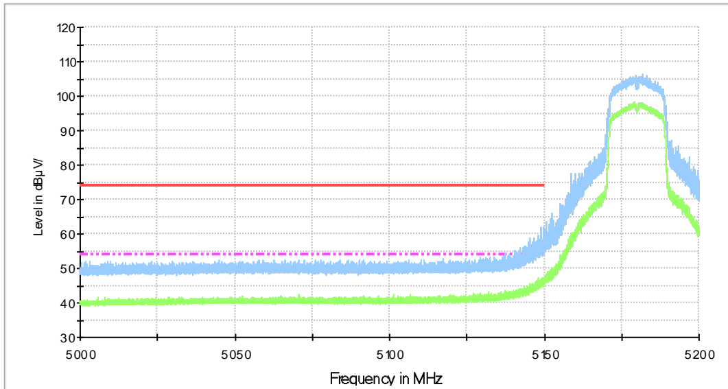
Fig.38 Band Edges (802.11n-HT20, 5180MHz)
