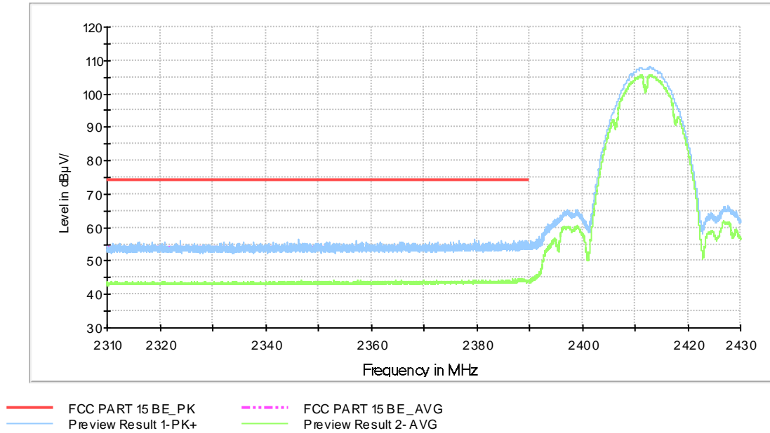
Fig.A.5.2.1 Radiated band Edges (802.11b, Ch 1)
