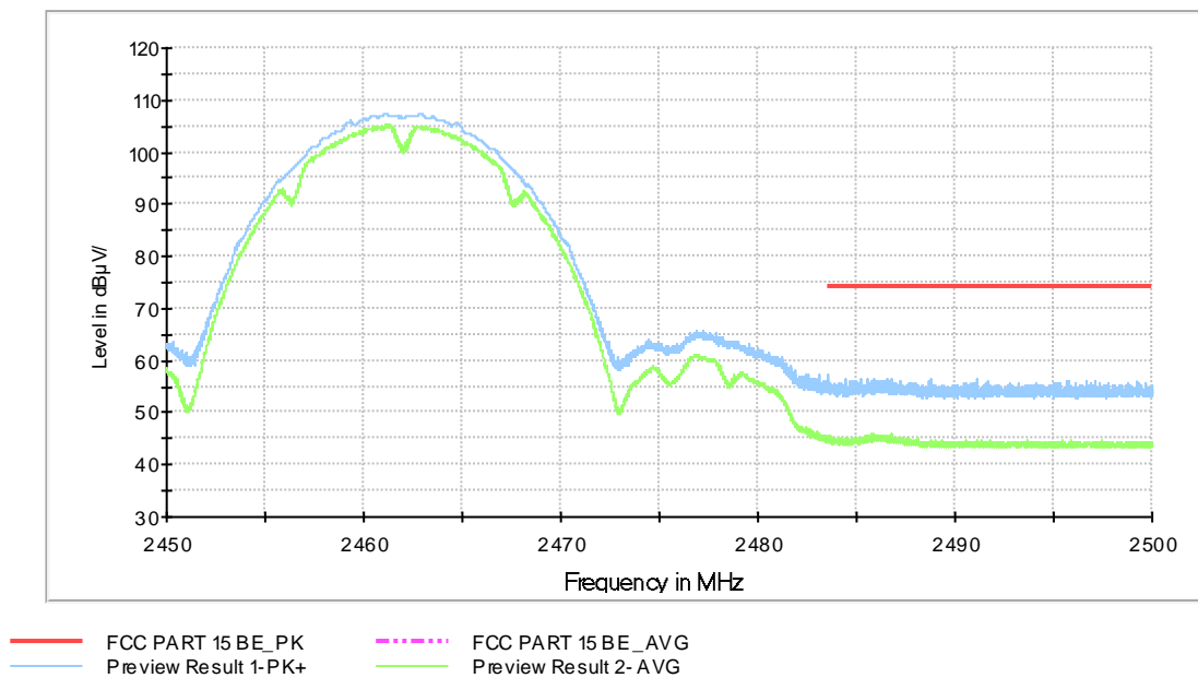
Fig.A.5.2.2 Radiated band Edges (802.11b, Ch 11)
