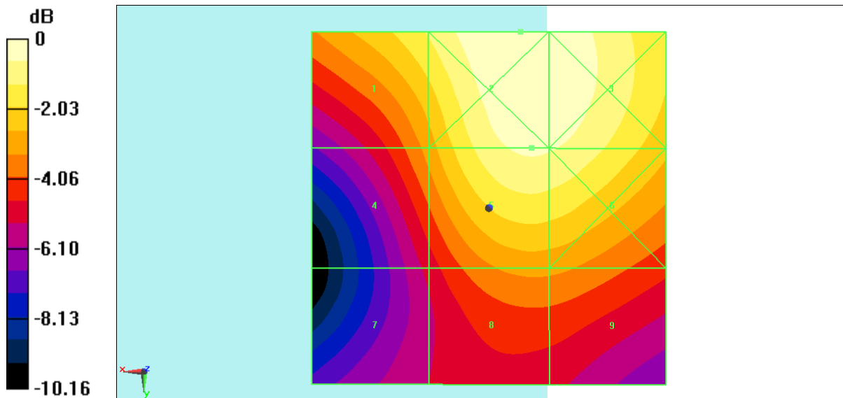
Fig B.4 HAC RF E-Field LTE Band41 PC3 QPSK CH39750
