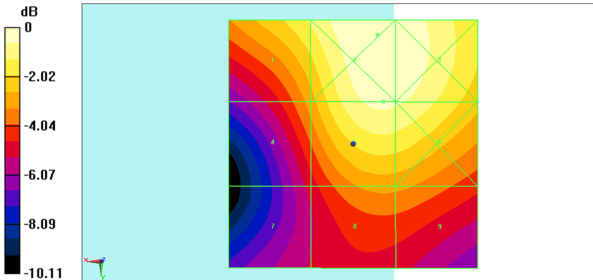
Fig B.3 HAC RF E-Field LTE Band41 PC2 QPSK CH39750
