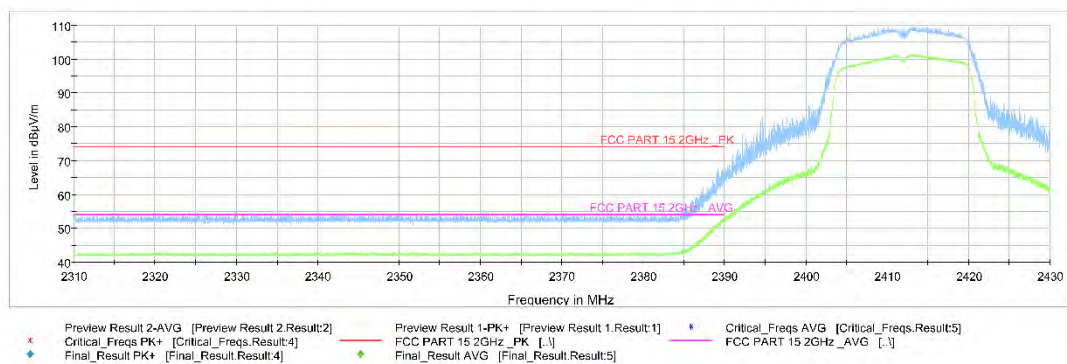
Fig.A.6.2.3 Transmitter Spurious Emission - Radiated (Power): 802.11g, ch1, 2.31 GHz - 2.43GHz
