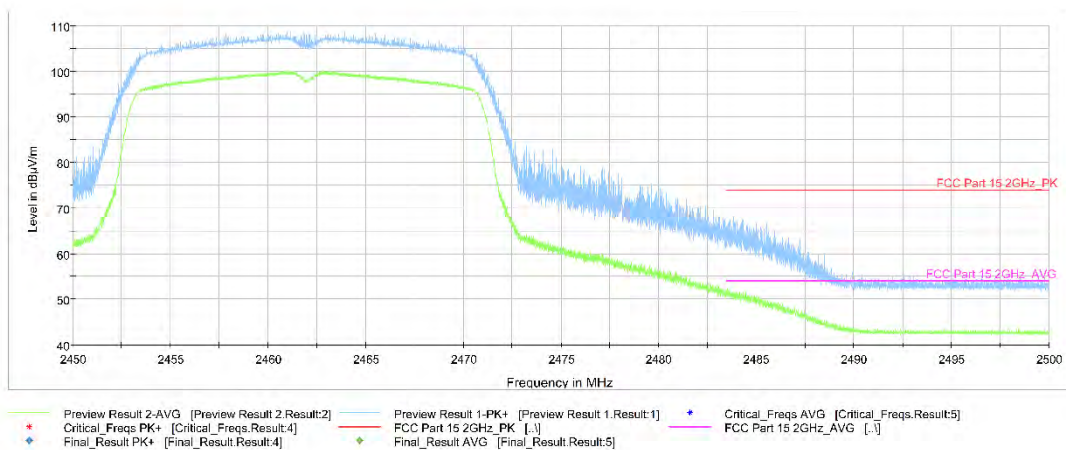
Fig.A.6.2.6 Transmitter Spurious Emission - Radiated (Power): 802.11n-HT20, ch11,
