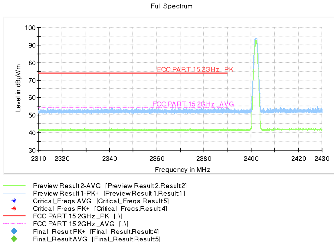
Fig.3. Frequency Band Edges: GFSK, 2402 MHz, Hopping Off, 2.31 GHz – 2.43GHz
