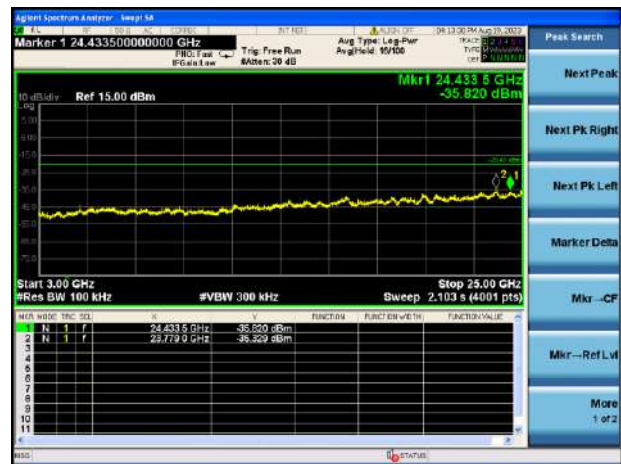
\pi/4 -DQPSK MIDDLE CHANNEL, SPURIOUS 3 GHz ~ 25 GHz
