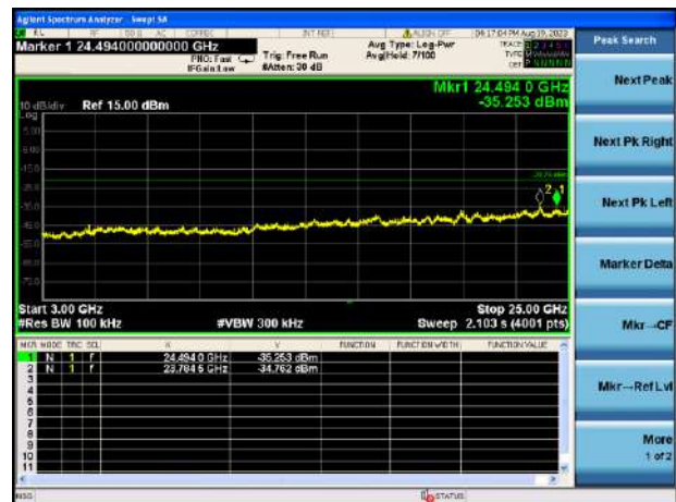
\pi/4 -DQPSK HIGH CHANNEL, SPURIOUS 3 GHz ~ 25 GHz
