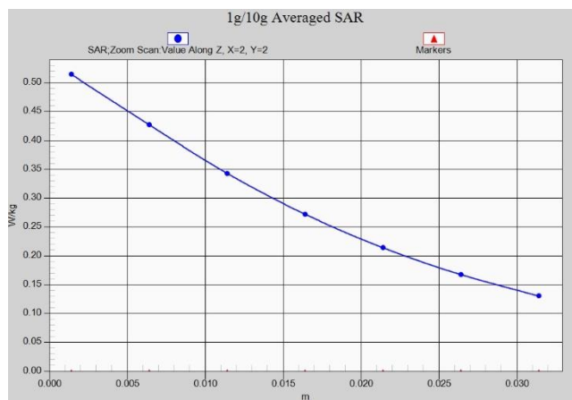
Fig. 1-14 Z-Scan at power reference point (WCDMA850 MHz Body)
