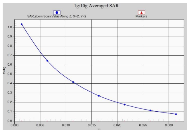
Fig. 1-15 Z-Scan at power reference point (LTE B2 MHz Body)
