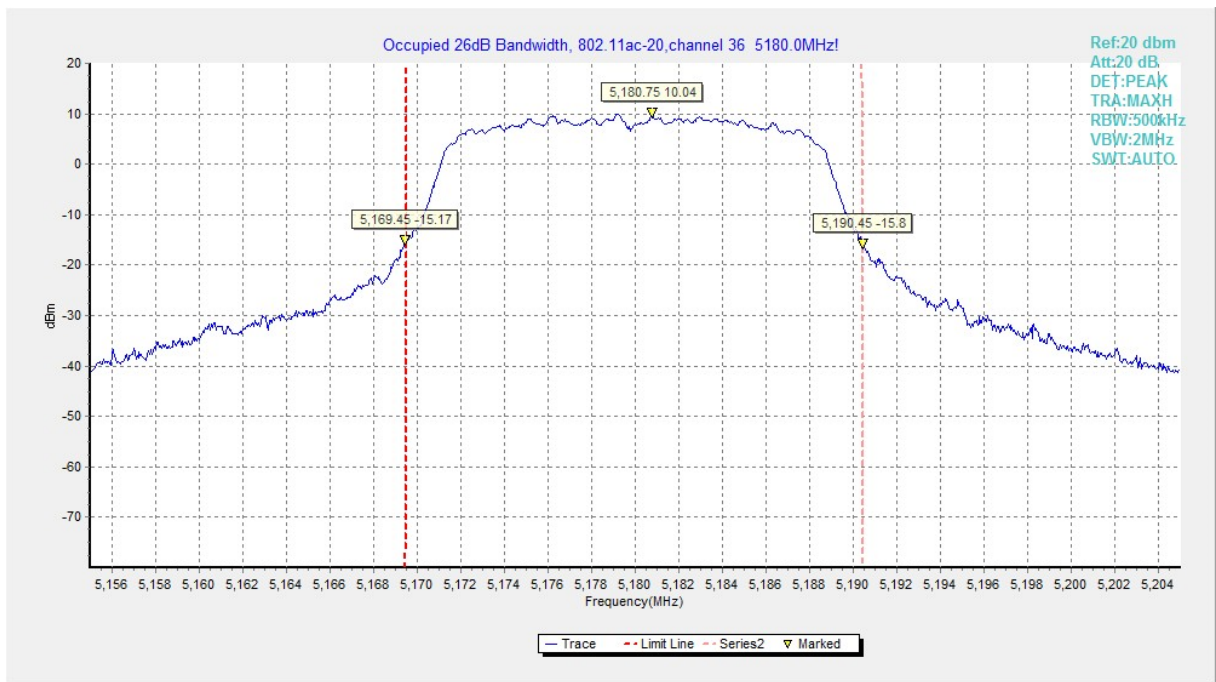
Fig.19 Occupied 26dB Bandwidth (802.11ac-HT20, 5180MHz)
