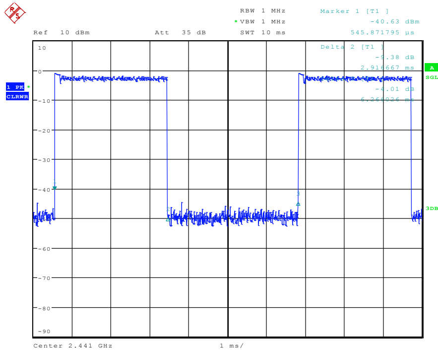
Fig. 101 Duty cycle: \pi/4 DQPSK Channel 39
