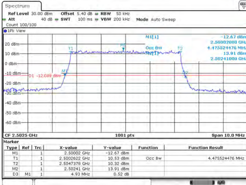
Band7-5MHz-QPSK-20775-25RB#0-4.476
