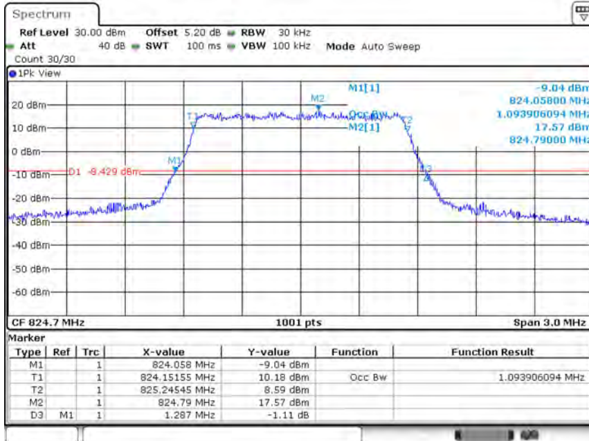
Band5-1.4MHz-QPSK-20407-6RB#0-1.094
