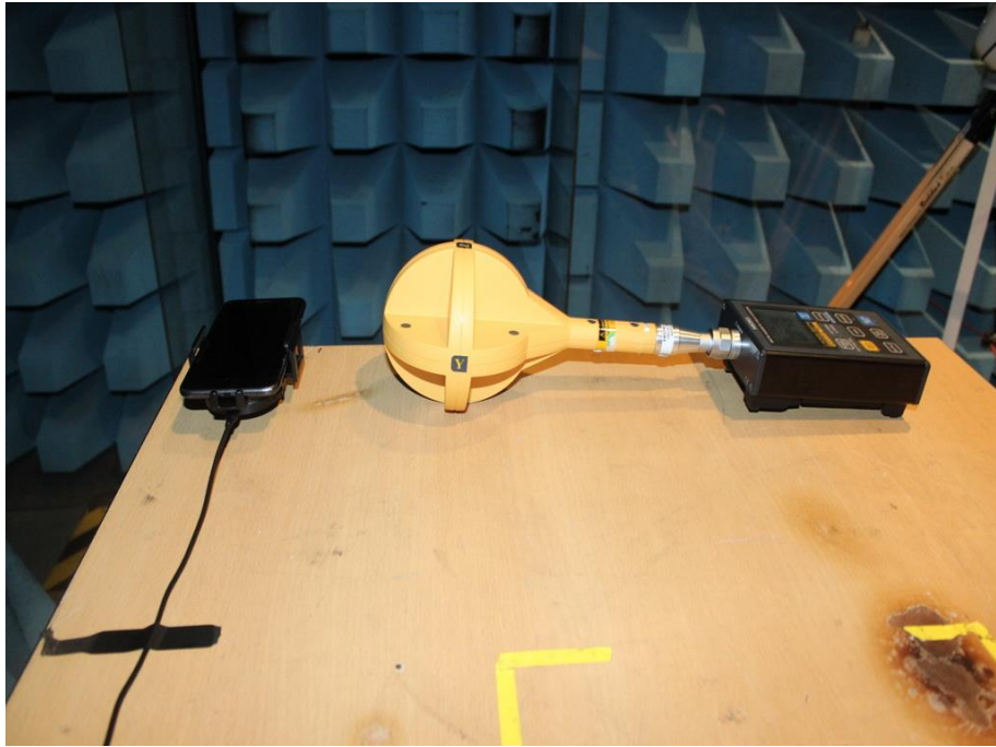
Photograph 3: Set-up for RF Exposure
