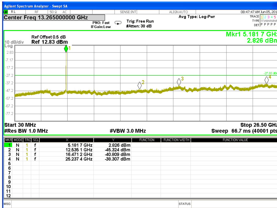
TX Spurious Emissions 802.11ac(HT20) Mode CH 36
