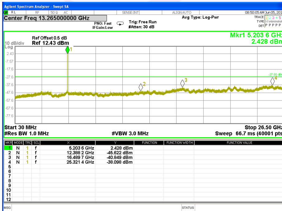
TX Spurious Emissions 802.11ac(HT20) Mode CH 40
