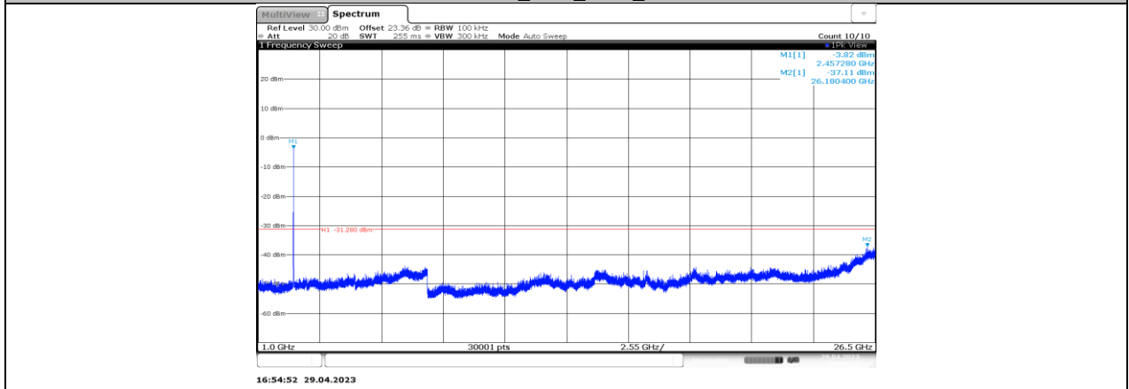
11N20SISO_Ant1_2462_1000~26500
