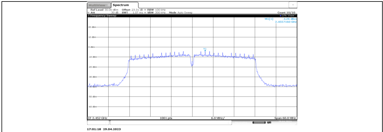
11N40SISO_Ant1_2452_0~Reference
