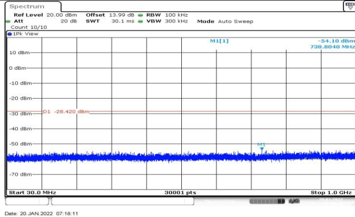
11N20SISO_Ant1_2412_30~1000
