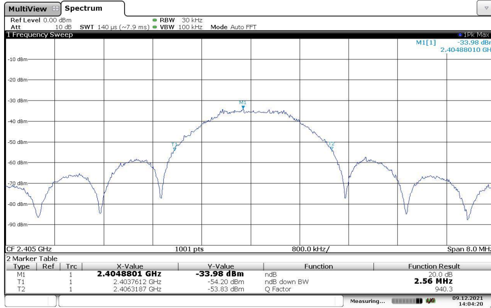
20 dB BANDWIDTH LOW CH
