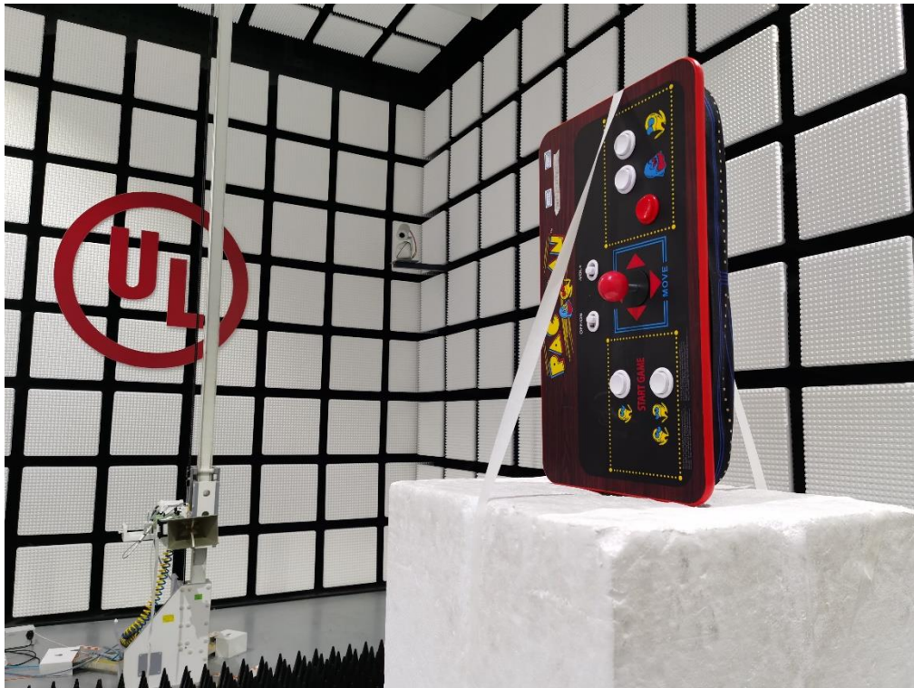
Radiated Disturbance above 1 GHz (Above 1G – Z axis)
