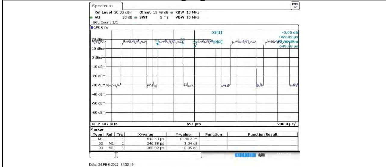
11N20SISO Ant1 2437
