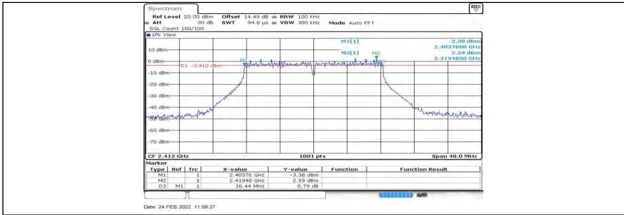
11N20SISO Ant1_2412
