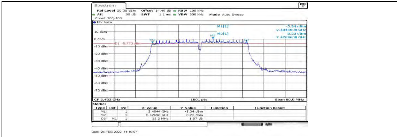
11N40SISO Ant1_2422
