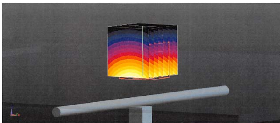
0 dB = 2.78 W/kg = 4.44 dBW/kg
