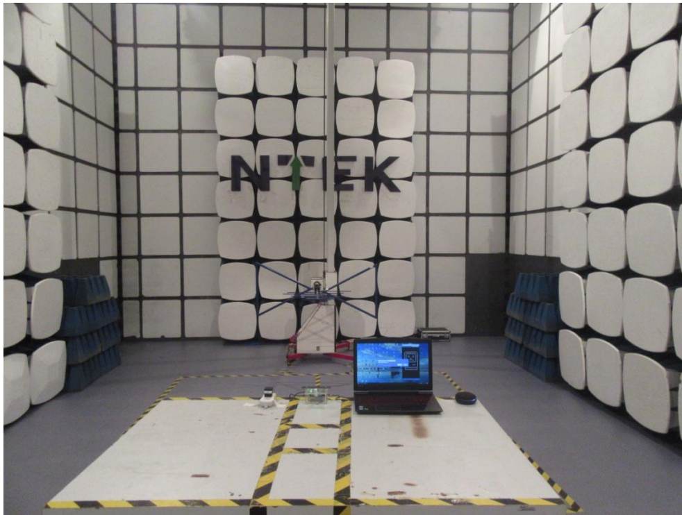
Radiated Measurement Photos (Model: DDKL4Q1)
